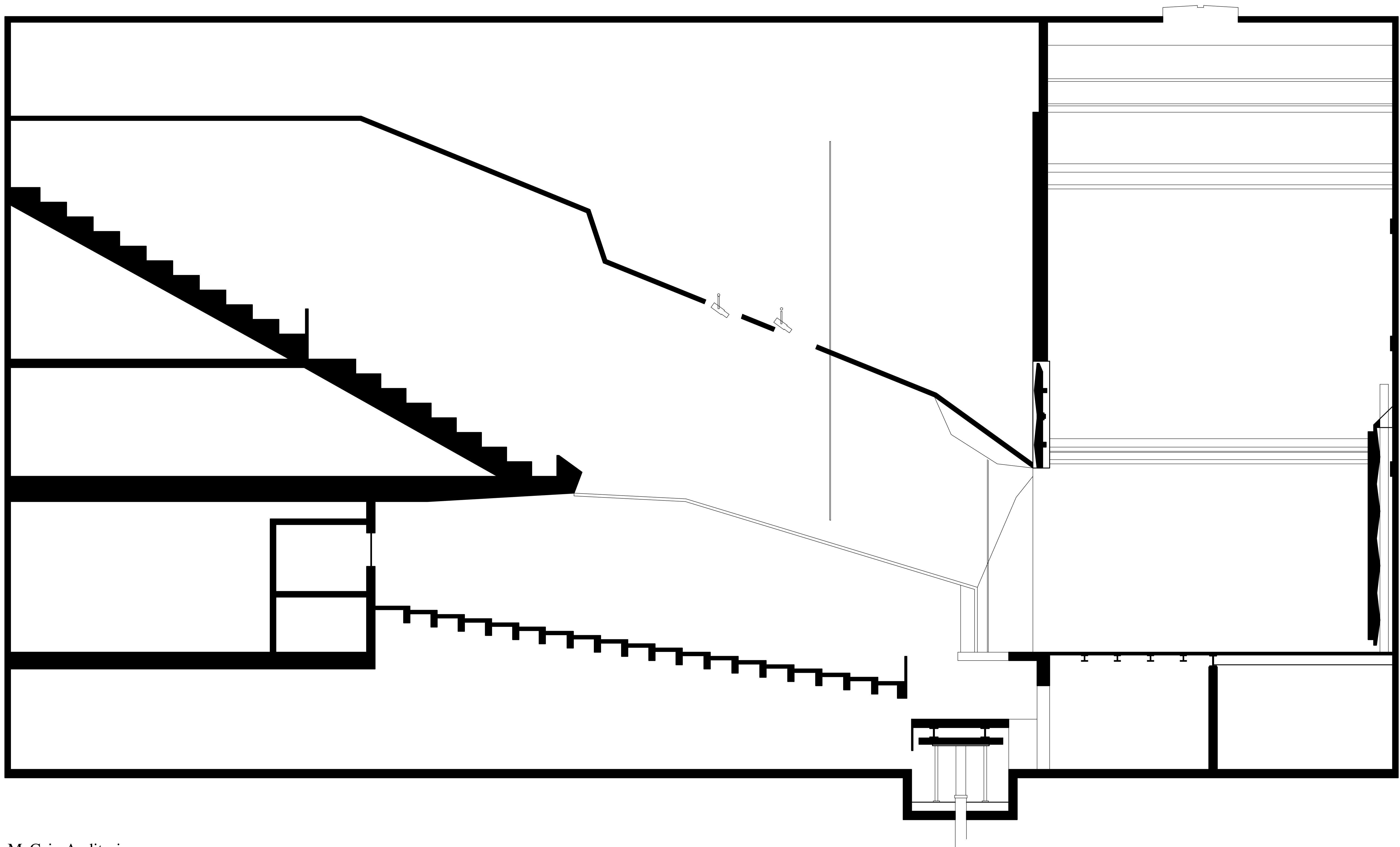
McCain Auditorium Kansas State University Scale: 3/16"=1'-0" when printed on 24x36 paper
