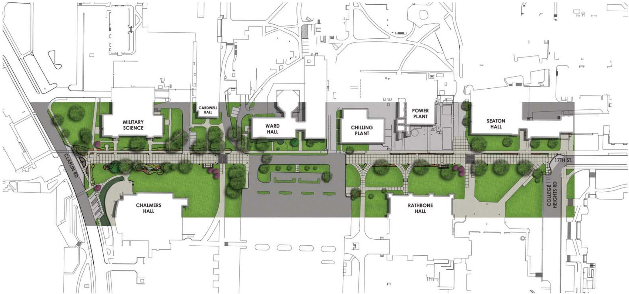
17TH STREET SITE PLAN
