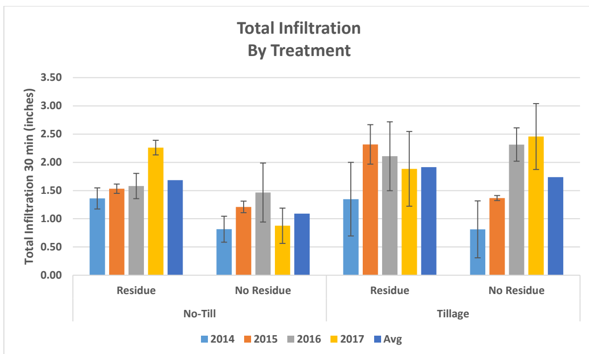
Figure 2. Measured infiltration over 30 minutes for tillage and residue management.
