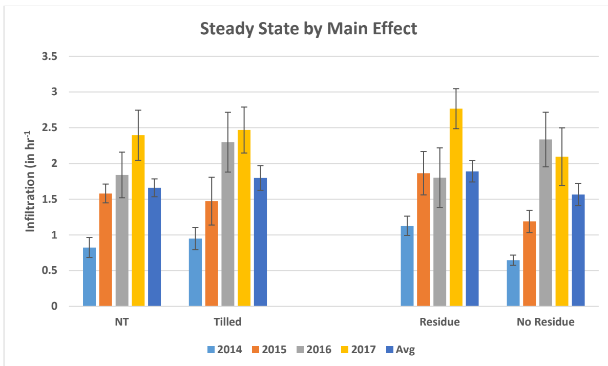
Figure 3. Impact of tillage and residue management on steady state infiltration.
