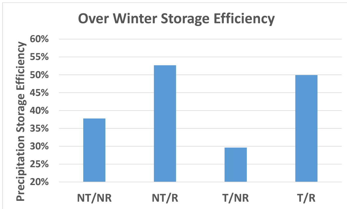
Figure 5. Precipitation storage efficiency from Oct 1, 2016 to May 30, 2017.
