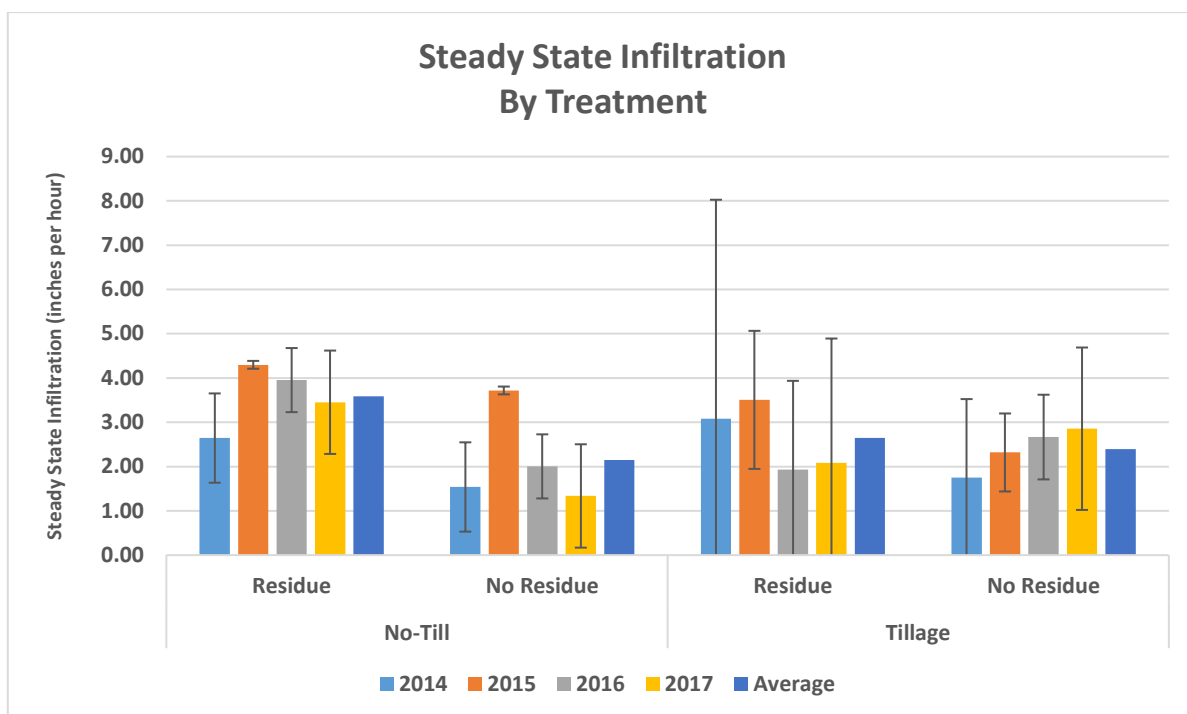
Figure 4. Steady state infiltration averaged over the last 4 measurements.
