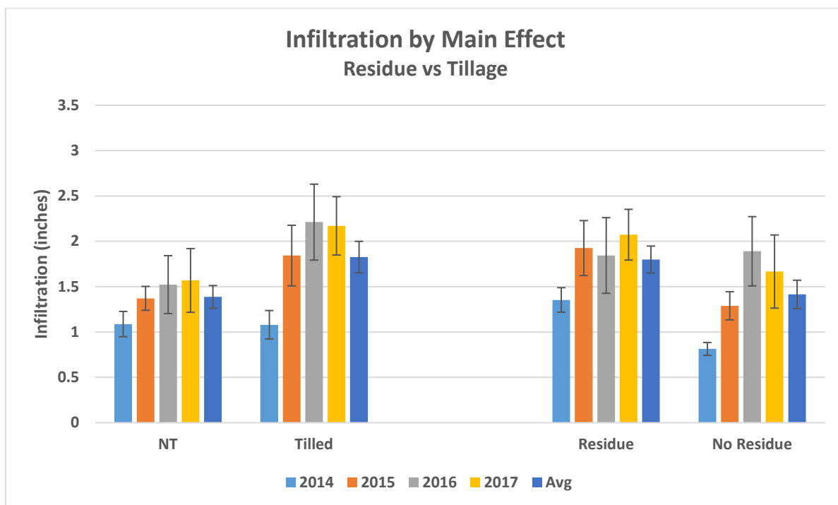
Figure 1. Impact of tillage and residue management on measured total infiltration.
