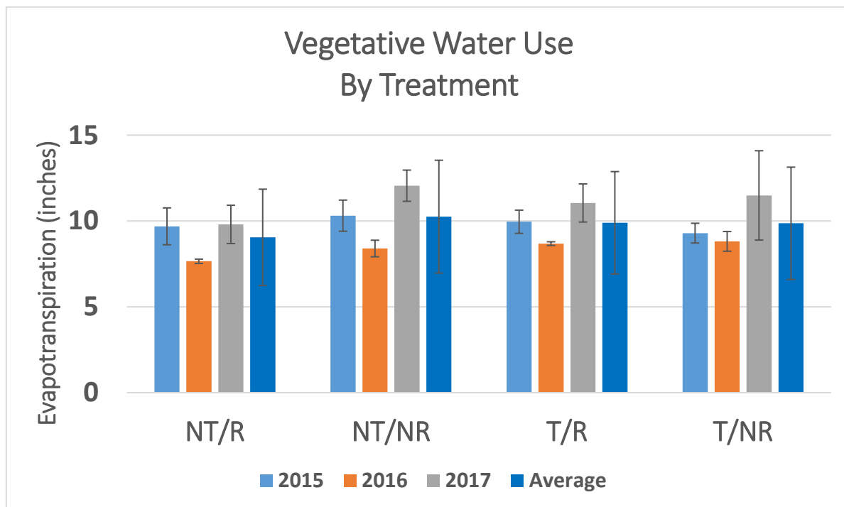
Figure 6. Vegetative water use by treatments for 2015 to 2017 and average.
