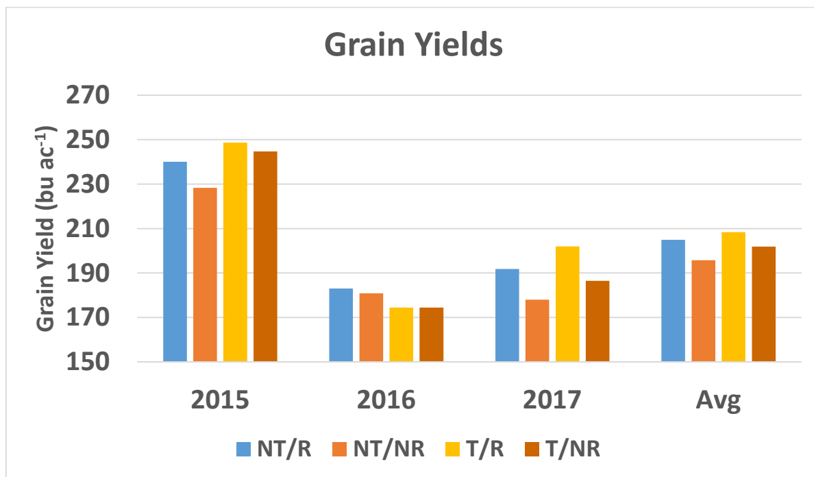
Figure 5. Grain yields for 2015, 2016 and 2017 by tillage and residue management. Average of nitrogen applications.
