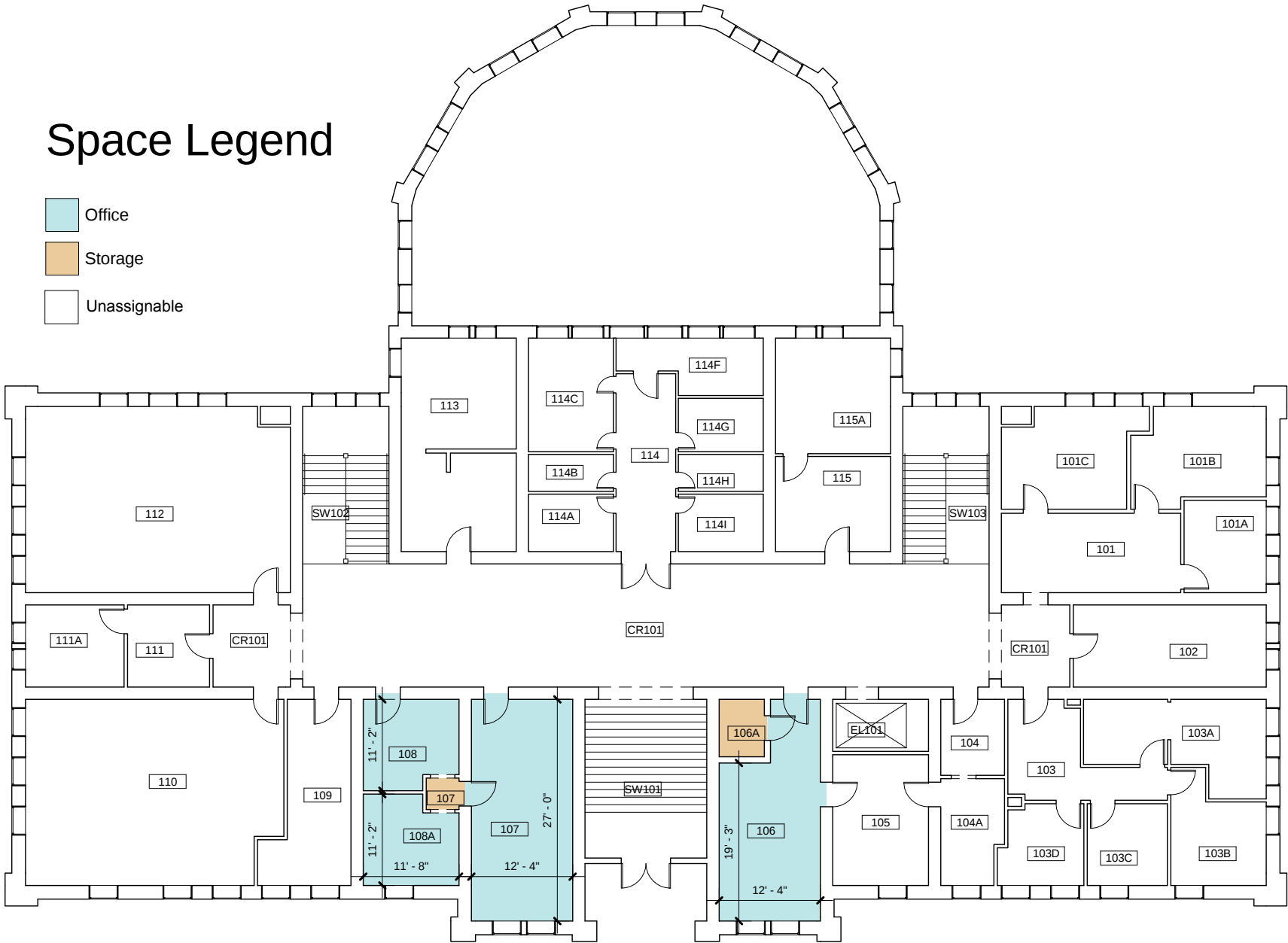
1 First Floor Plan 1/16" = 1'-0"
