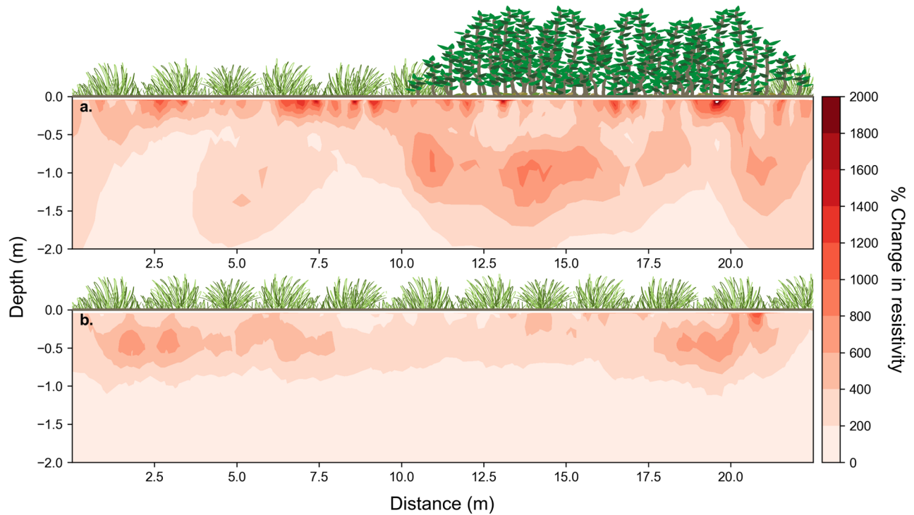
Figure 5. Change in ER from June 29 to October 3, 2022 at the (a) woody-encroached (N4D) and (b) grass transects (N1B). An increase in the inverted resistivity indicates a decrease in soil moisture. The upper 2 m of the woody-encroached transect exhibited a larger increase in soil drying (higher percent change in resistivity) compared to the grass transect.
