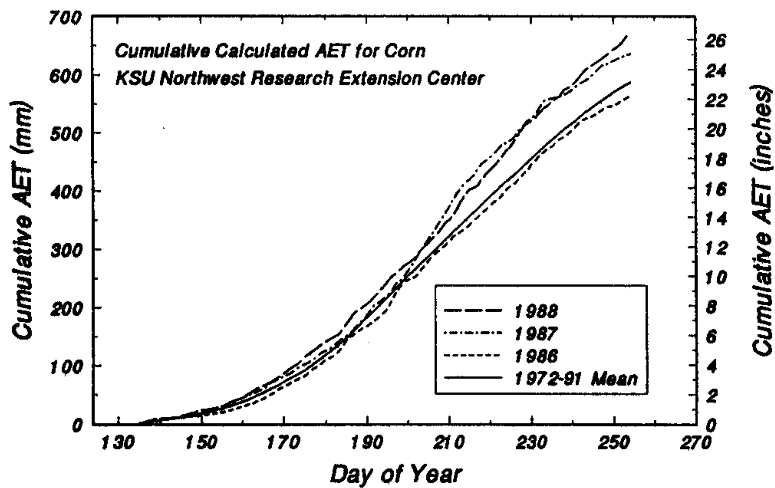
Figure 2—Cumulative calculated water use (AET) of corn for 1986 to 1988 and the long term mean (1972 to 1991) at Colby, Kansas.
