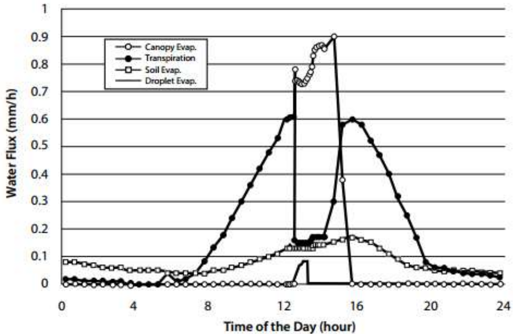
Figure 1. Water use for a rotator sprinkler placed on top of the pivot lateral irrigating at noon for 50 minutes. The figures illustrates, in addition to how water is lost during the irrigation, that crop transpiration occurs during daylight hours, while soil water evaporation occurs throughout the entire day. (Martin et al., 2012).
