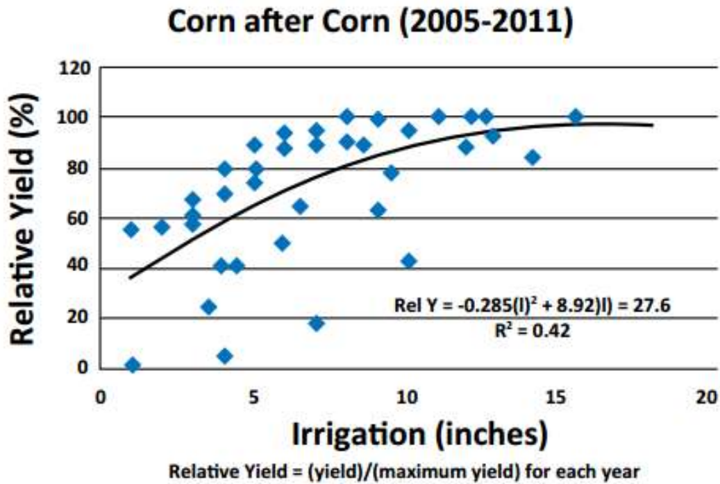
Figure 11. Relative Corn yield as related to irrigation amount for Garden City, KS. (Klocke, et al., 2015).
