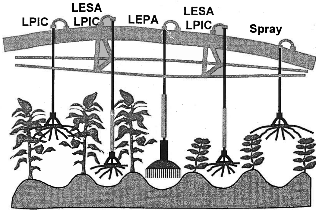
Figure 4. Illustration of the LEPA, LESA, LPIC, and spray application concepts in tall and short crops. The illustration has drops in each furrow to conserve space while actual systems typically use drops in alternate furrows either 60-in. or 80-in. (1.5-m or 2-m) apart depending on the crop row spacing.
