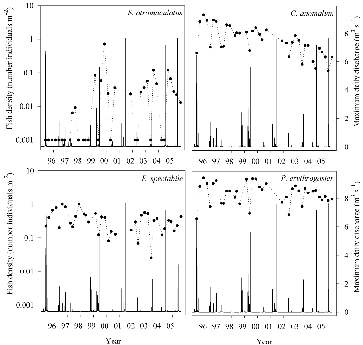
Fig. 5 Fish density (number of individuals m -2 ; left axis and dashed line) and maximum daily discharge (m 3 s -1 ; right axis and solid line) from a deep headwater site 1995–2005 on Kings Creek, Riley County, KS, U.S.A. Fish densities have had 0.001 added to facilitate plotting on a log plot.
