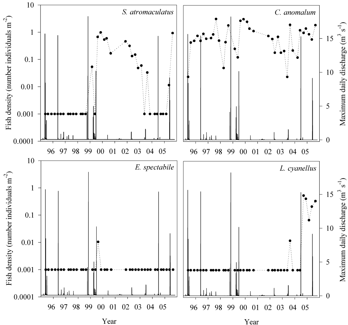
Fig. 4 Fish density (number of individuals m -2 ; left axis and dashed line) and maximum daily discharge (m 3 s -1 ; right axis and solid line) from a shallow headwater site 1995–2005 on Kings Creek, Riley County, KS, U.S.A. Fish densities have had 0.001 added to facilitate plotting on a log plot.
