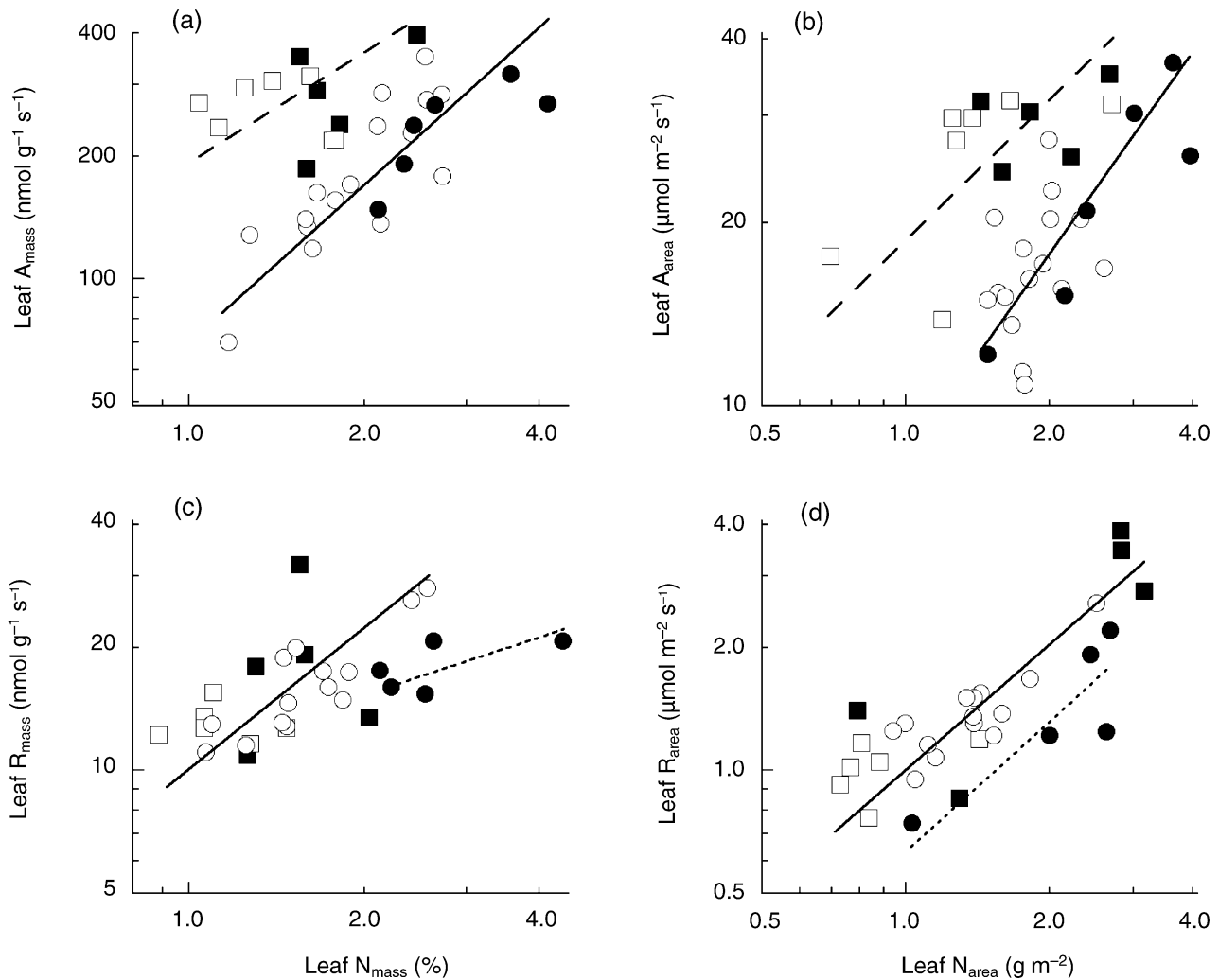
Fig. 1 Leaf trait relationships among 39 savannah species. Species means are shown identified as forbs ( \circ ), legumes ( \bullet ), C_3 grasses ( \blacksquare ), and C_4 grasses ( \square ). Note the \log_{10} scale. Type II regression lines illustrate a posteriori group contrasts among species. (a) A_{\text{mass}} - N_{\text{mass}} correlations for the combined C_3 and C_4 grass groups ( r = 0.20 , P = 0.52 , n = 12 ) and combined forb and legume groups ( r = 0.82 , P < 0.001 , n = 22 ). (b) A_{\text{area}} - N_{\text{area}} correlations for the combined C_3 and C_4 grass groups ( r = 0.62 , P = 0.03 , n = 12 ) and combined forb and legume groups ( r = 0.72 , P < 0.001 , n = 22 ). (c) R_{\text{mass}} - N_{\text{mass}} correlations for the legume group ( r = 0.63 , P = 0.26 , n = 5 ) and for the combined C_3 and C_4 grass and forb groups ( r = 0.64 , P < 0.001 , n = 25 ). (d) R_{\text{area}} - N_{\text{area}} correlations for the legume group ( r = 0.85 , P = 0.07 , n = 5 ) and for the combined C_3 and C_4 grass and forb groups ( r = 0.86 , P < 0.001 , n = 25 ).
